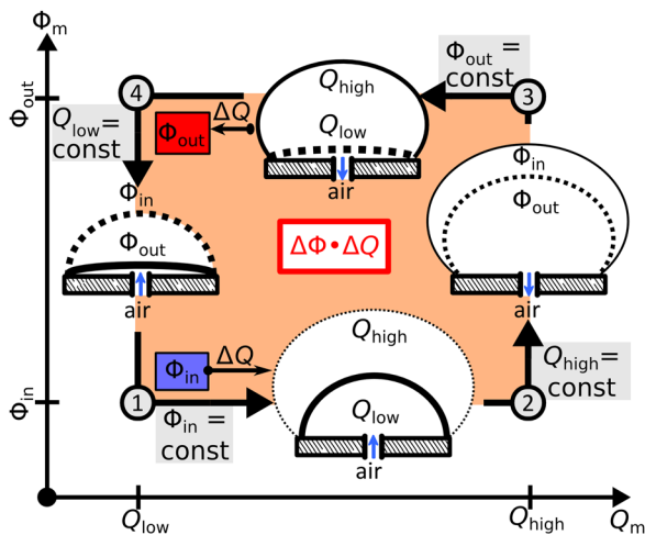
FIG. 2. (Color online) Rectangular energy conversion cycle operating between two charge reservoirs depicted in the work-conjugate ( \Phi, Q ) plane. The cycle proceeds counterclockwise from state 1 to state 4. During the four steps of the cycle solid and dashed lines indicate the evolution of the balloon shape. In the constant voltage steps, 1 \rightarrow 2 and 3 \rightarrow 4, charges are taken from the low voltage reservoir and fed into the high voltage reservoir. In the constant charge steps 2 \rightarrow 3 and 4 \rightarrow 1, the voltage across the membrane is brought in line with the reservoirs. The area enclosed by the contour corresponds to the generated electrical energy \Delta\Phi\Delta Q .
